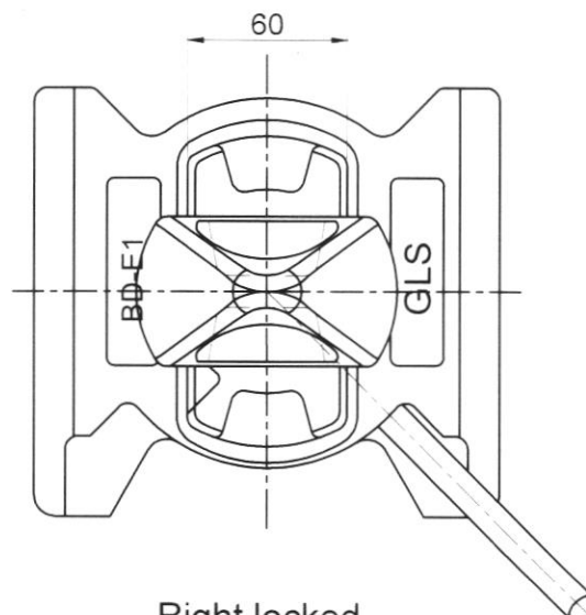
Right locked
