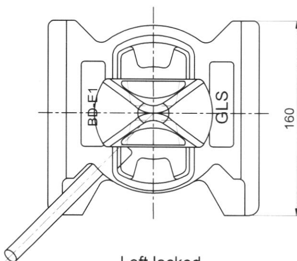
Left locked
