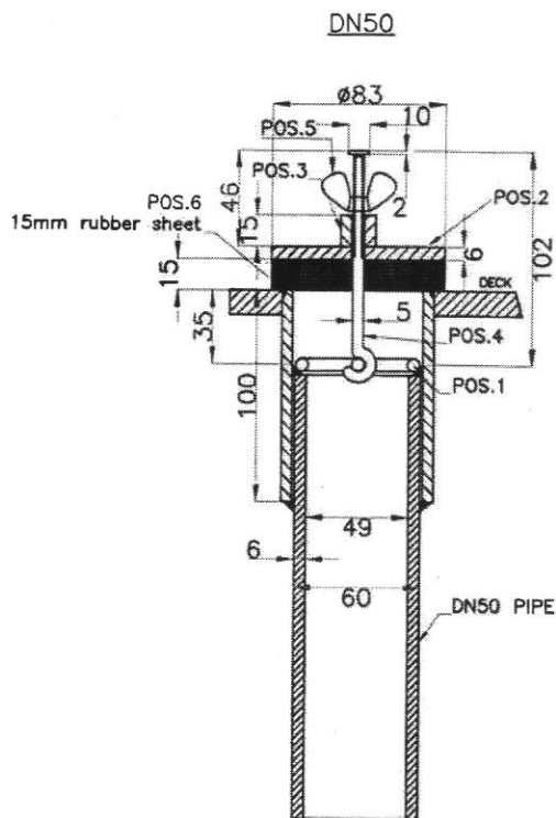
PROFILE
