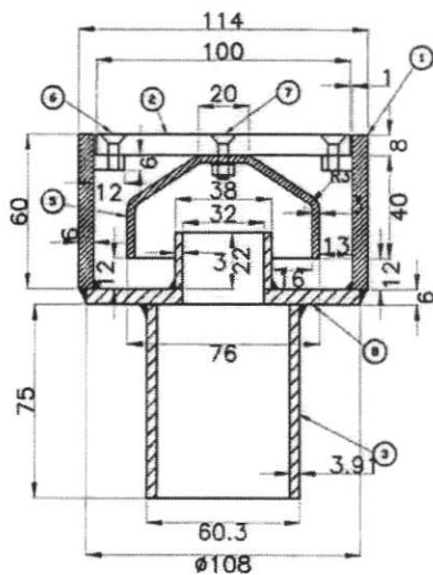
TANK DETAILS
