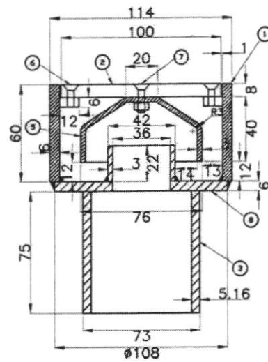
TANK DETAILS
