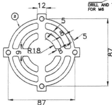
GRATING [COMMON FOR DN40&50]
