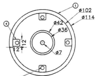
TANK DETAILS
