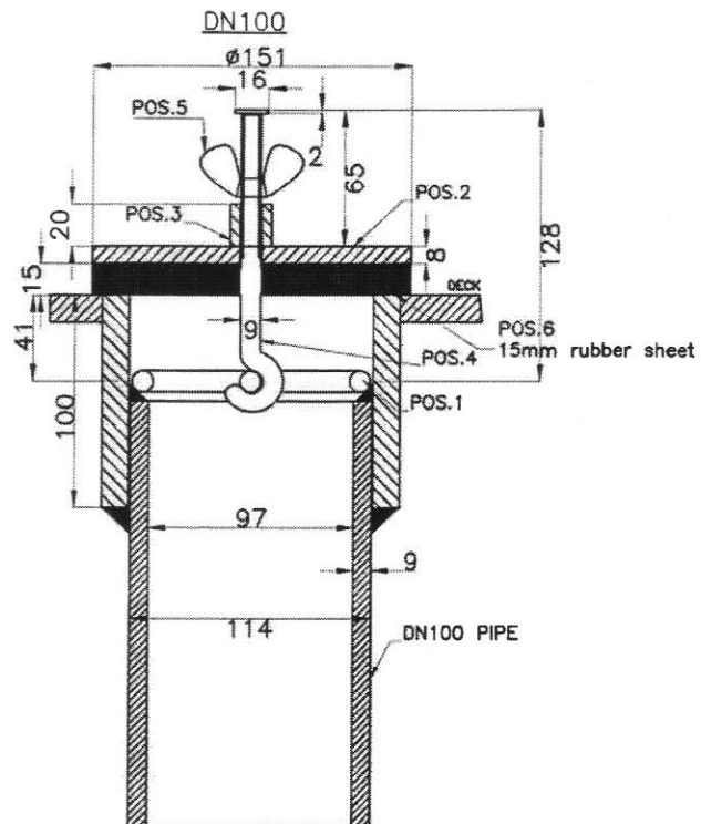
PROFILE
