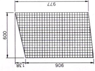
LADDER L19-L20 HOT DIP GALVANIZED STEEL QTY. 2
