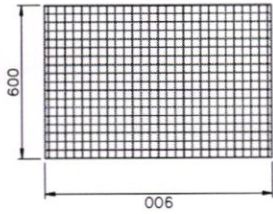
RAILING HOT DIP GALVANIZED STEEL QTY-9
