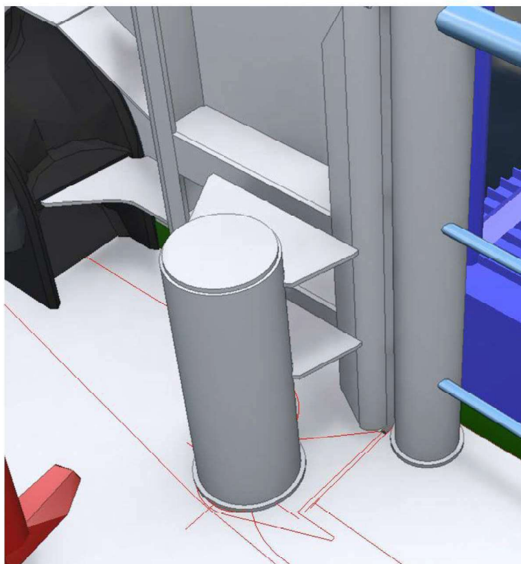
Fig 1- sample image of single fairlead roller in the vessel (indicative only)
