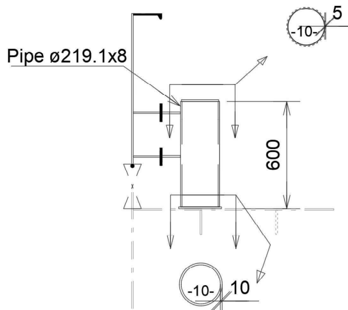
Fig 2- sample image of single fairlead roller in the vessel (indicative only)
