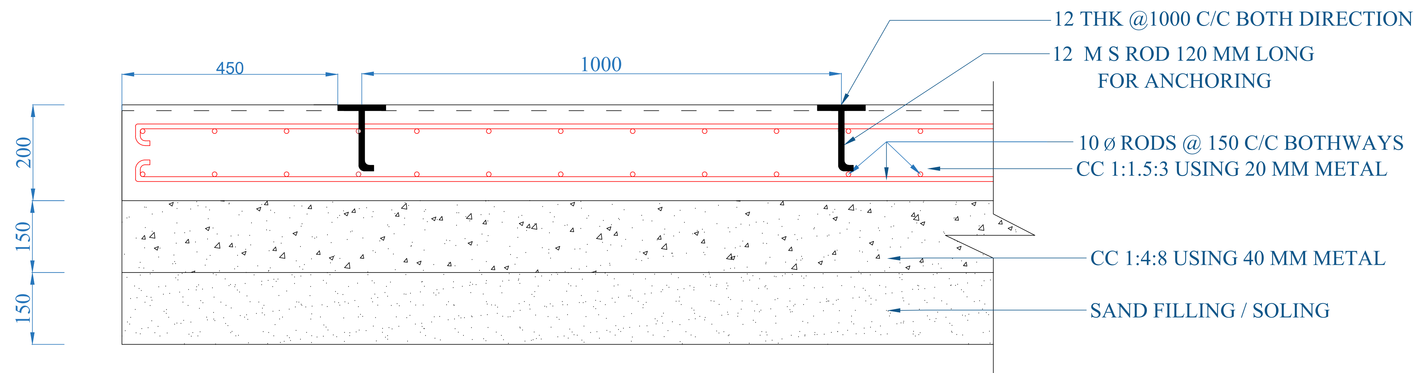
CROSS SECTION OF SKID
