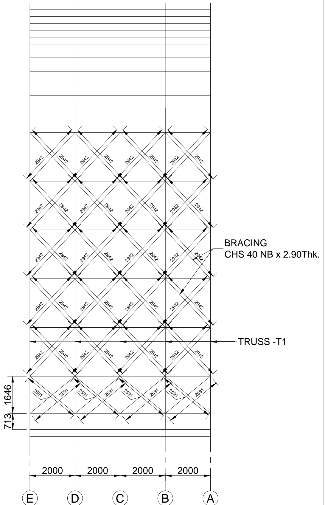
SIDE ELEVATION A - BOTTOM MEMBER
