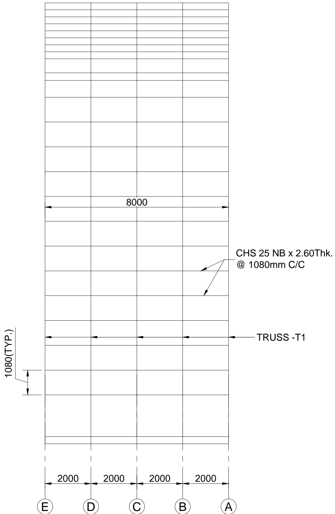
SIDE ELEVATION A - TOP MEMBER
