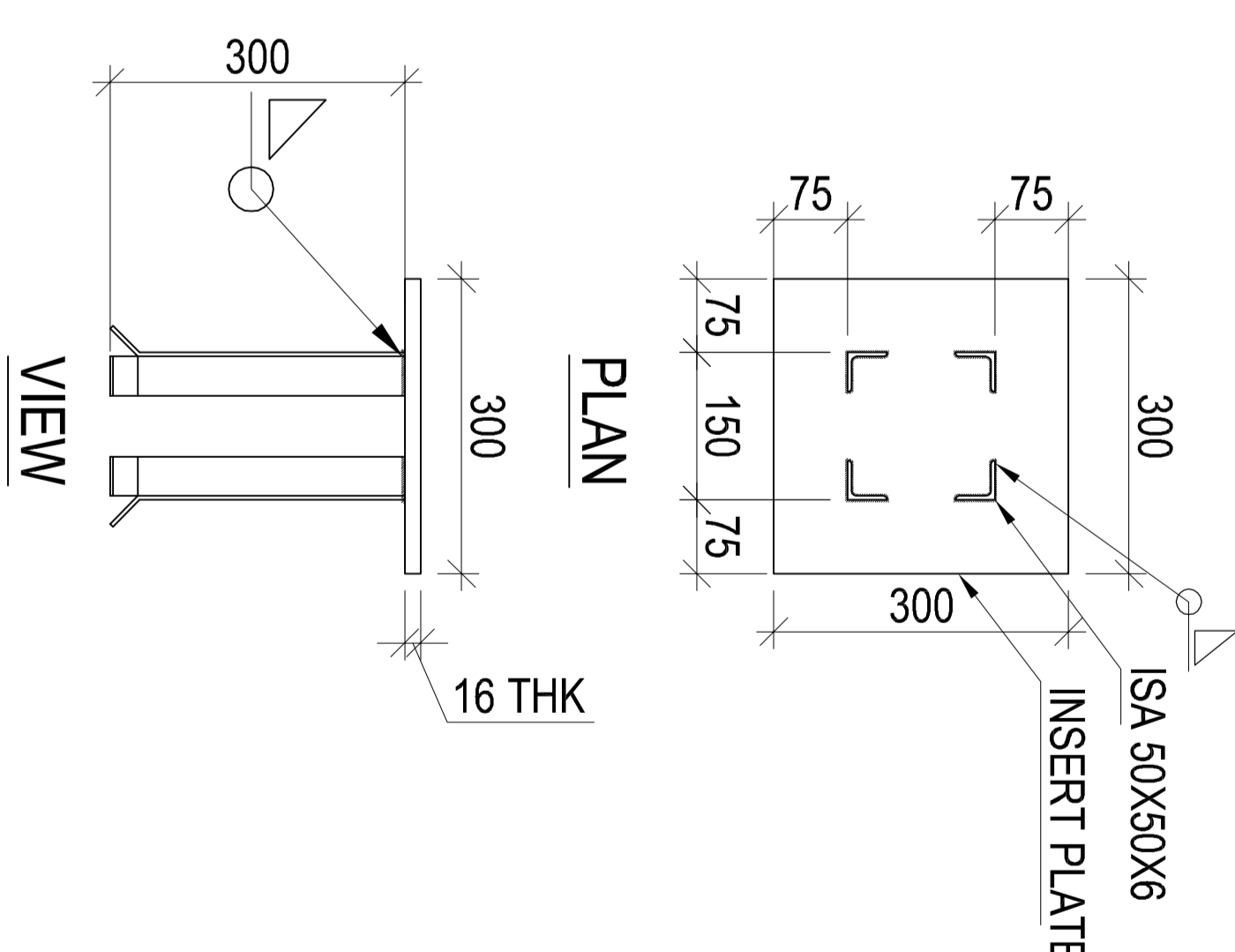
INSERT PLATE DETAIL IP -300X300X16 @1000 C/C
