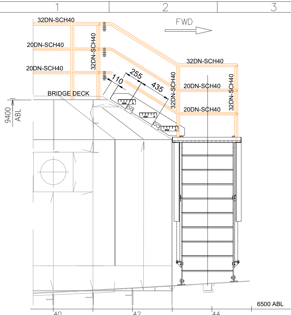
PROFILE VIEW LOOKING PORT
