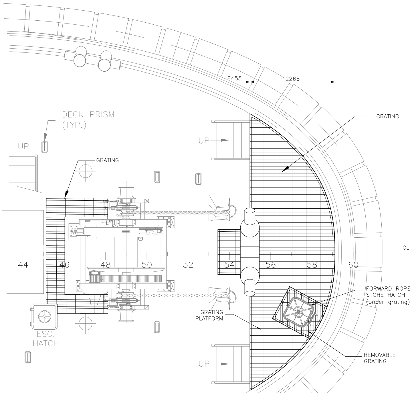
MAIN DECK PLAN SCALE : NTS
