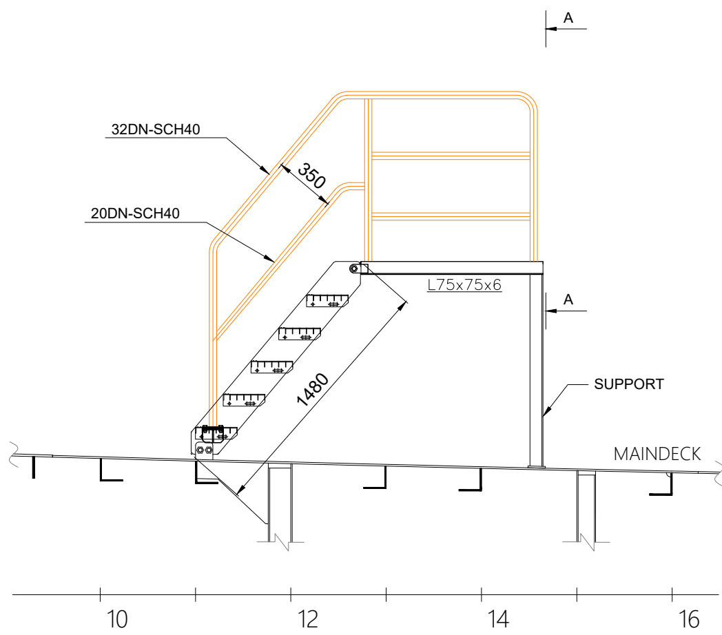
PROFILE VIEW PORT AND STBD SIMILAR
