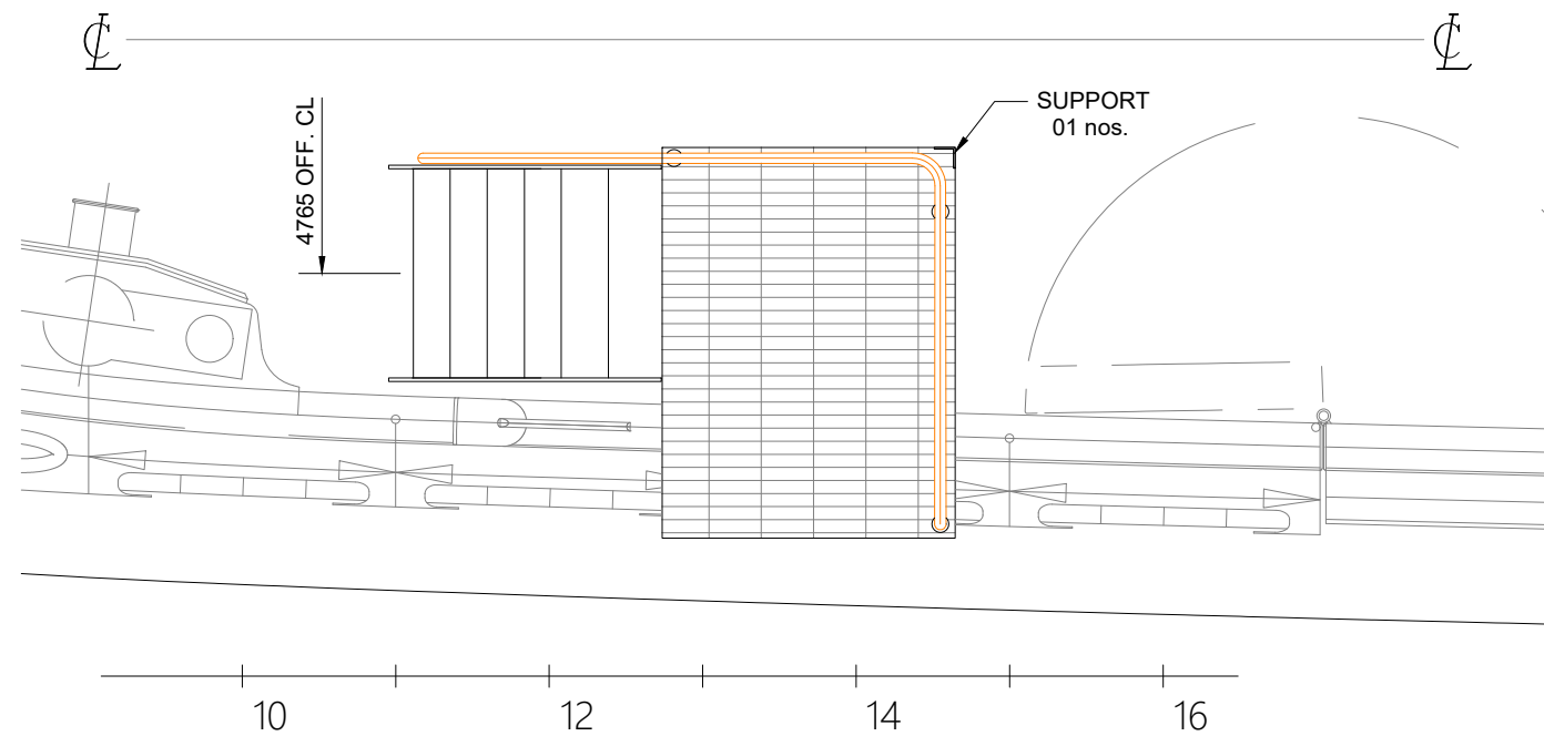
MAIN DECK PLAN VIEW PORT AND STBD SIMILAR
