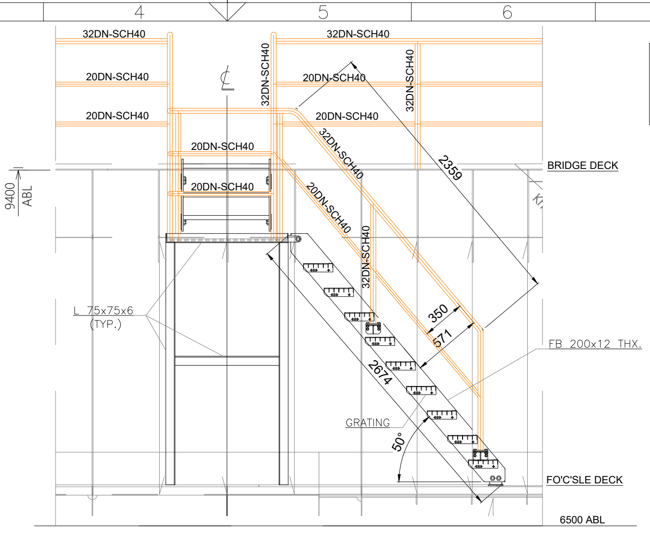
TRANSVERSE VIEW LOOKING AFT
