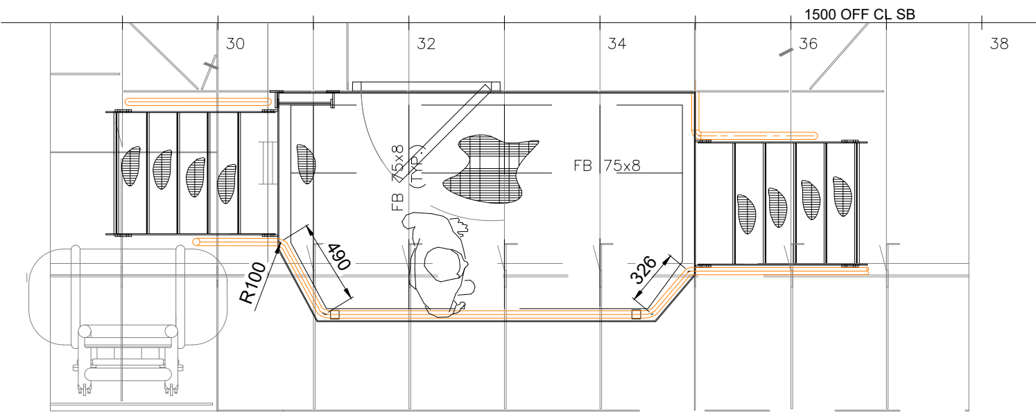
PLAN VIEW STBD SIDE SHOWN PORT SIDE SIMILAR
