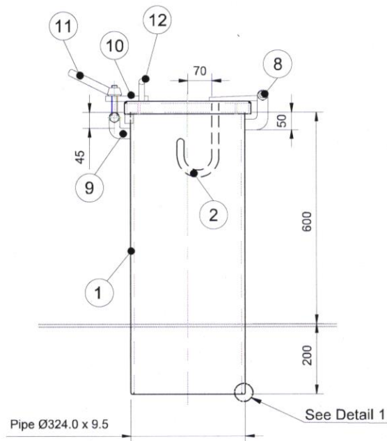
View section A-A
