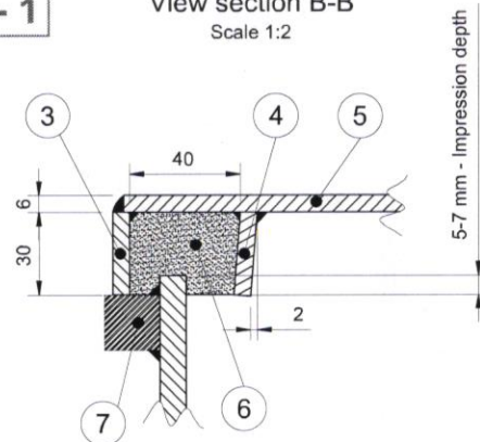
View section B-B
