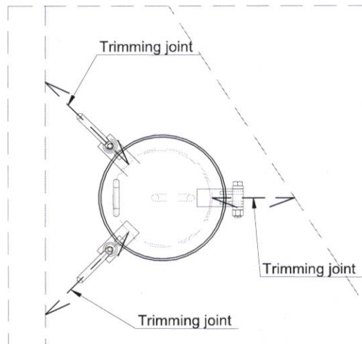
Installation example
