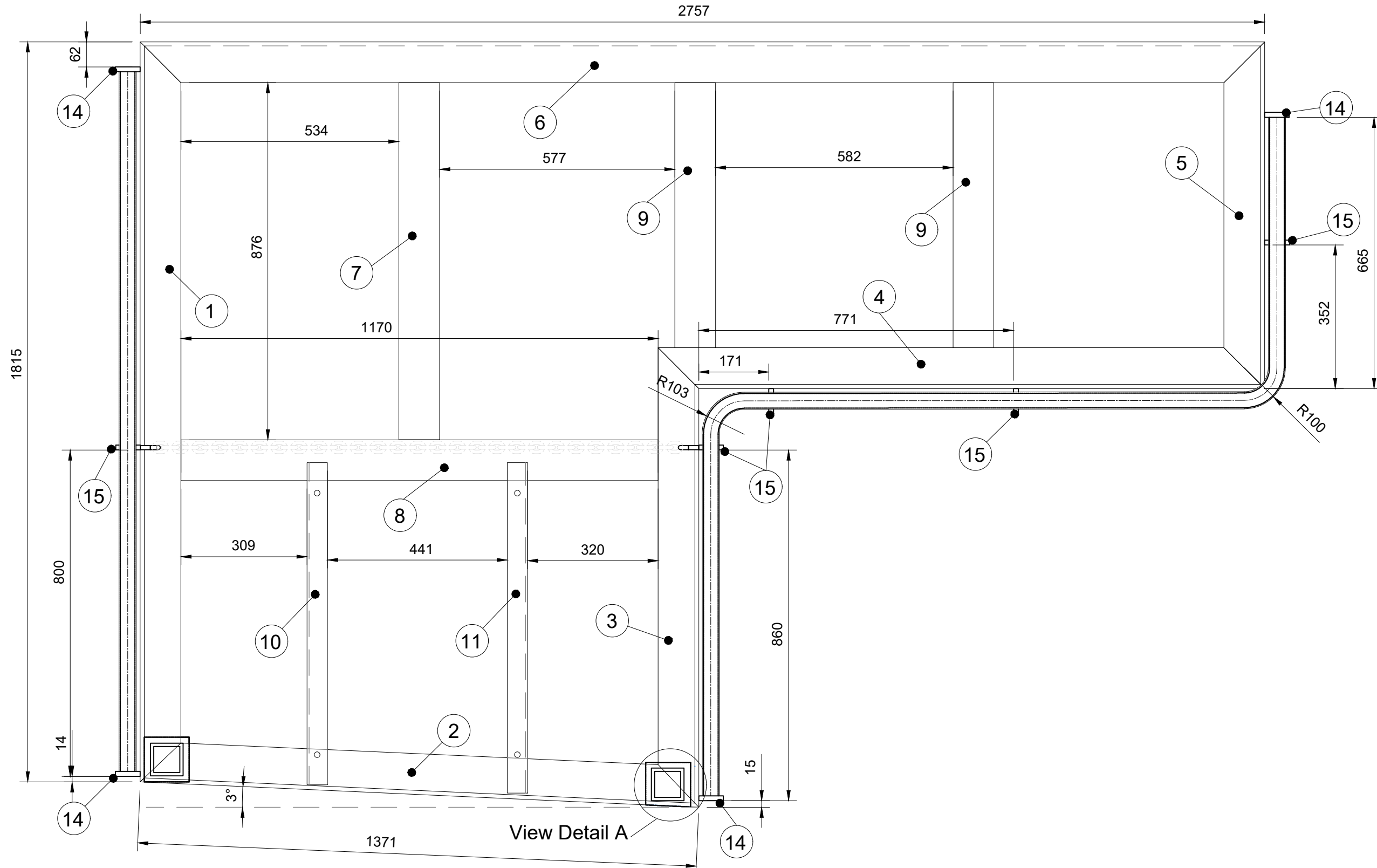
Scale 1:10
