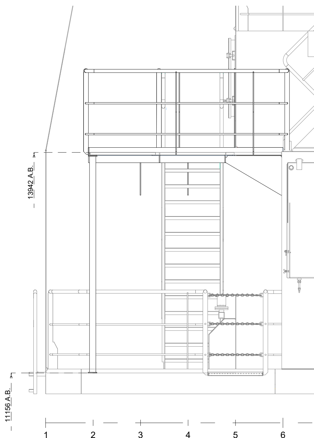
View section A-A
