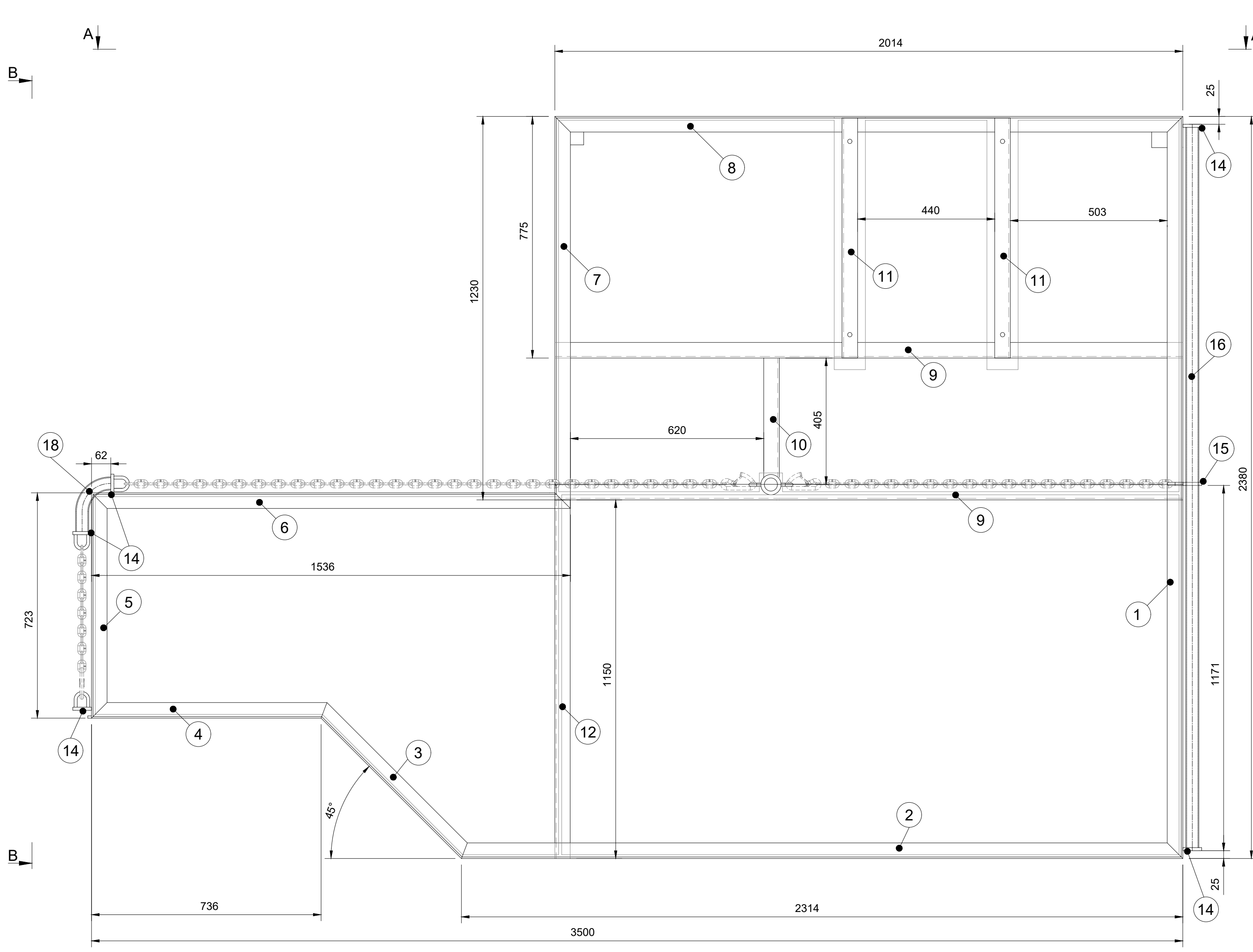
View B-B Scale 1:10
