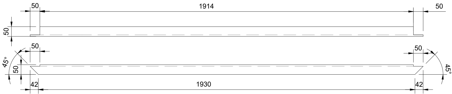
Detail Pos. 9 Scale 1:10
