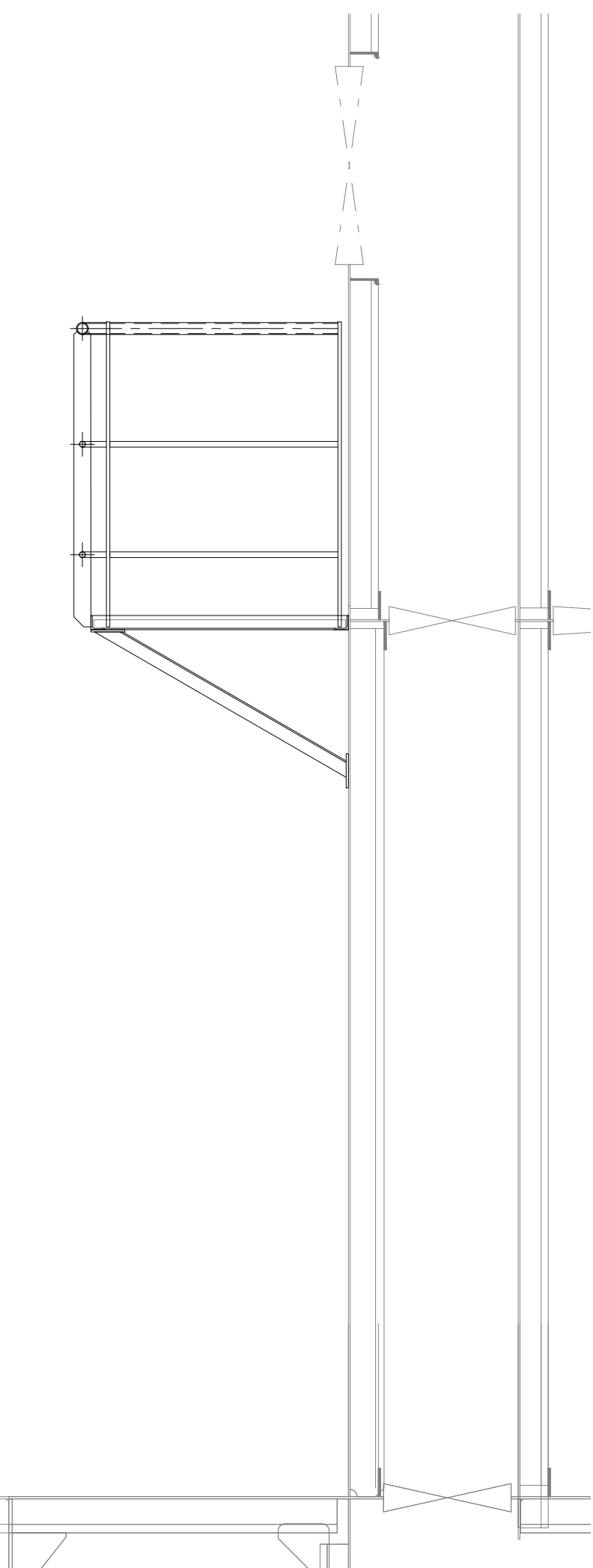
View section B-B
