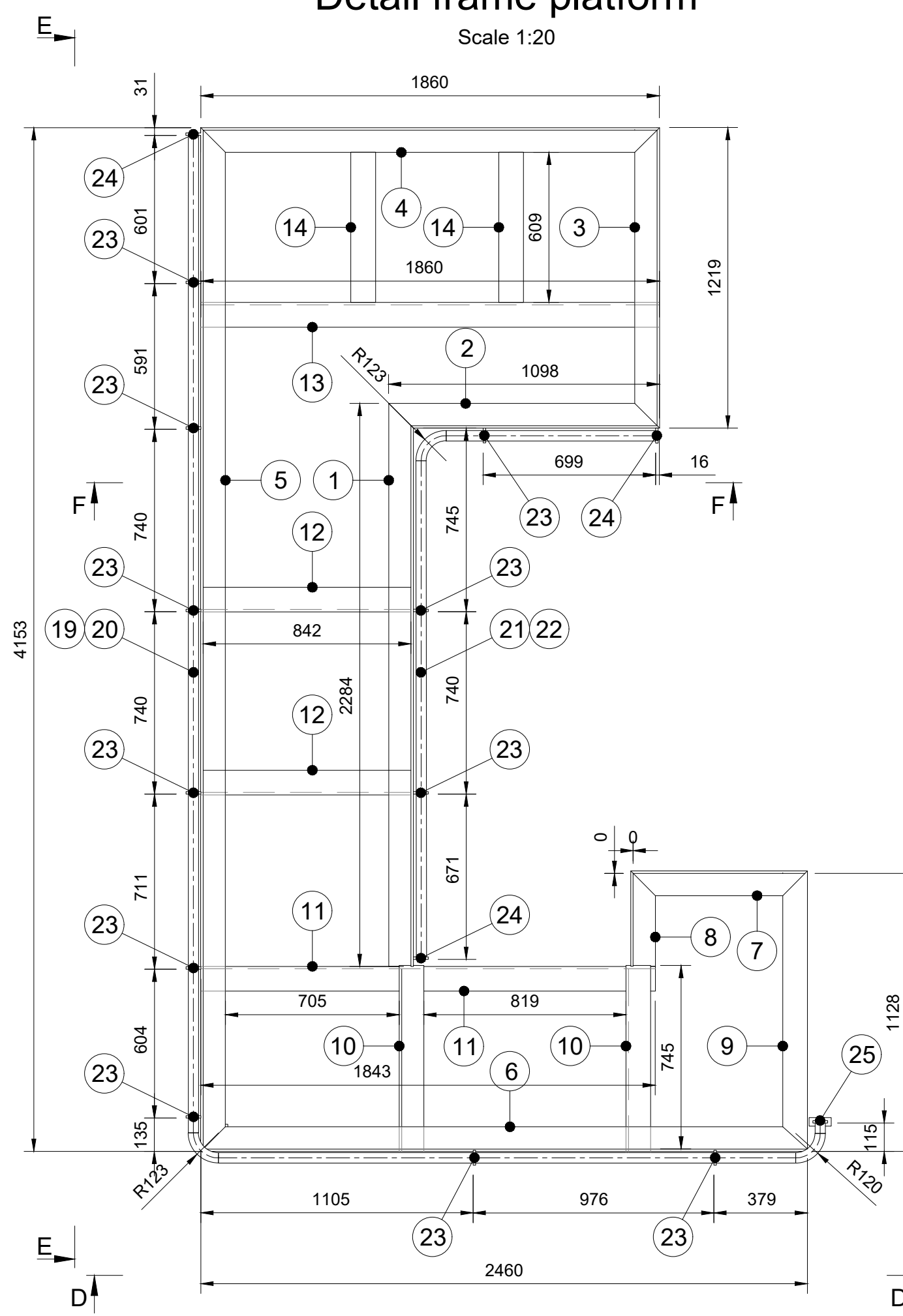
Detail frame platform
