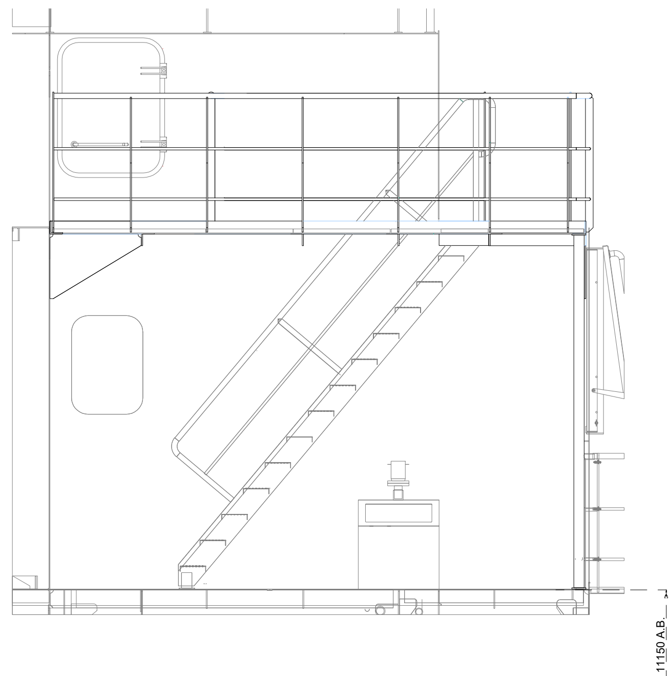
View section C-C
