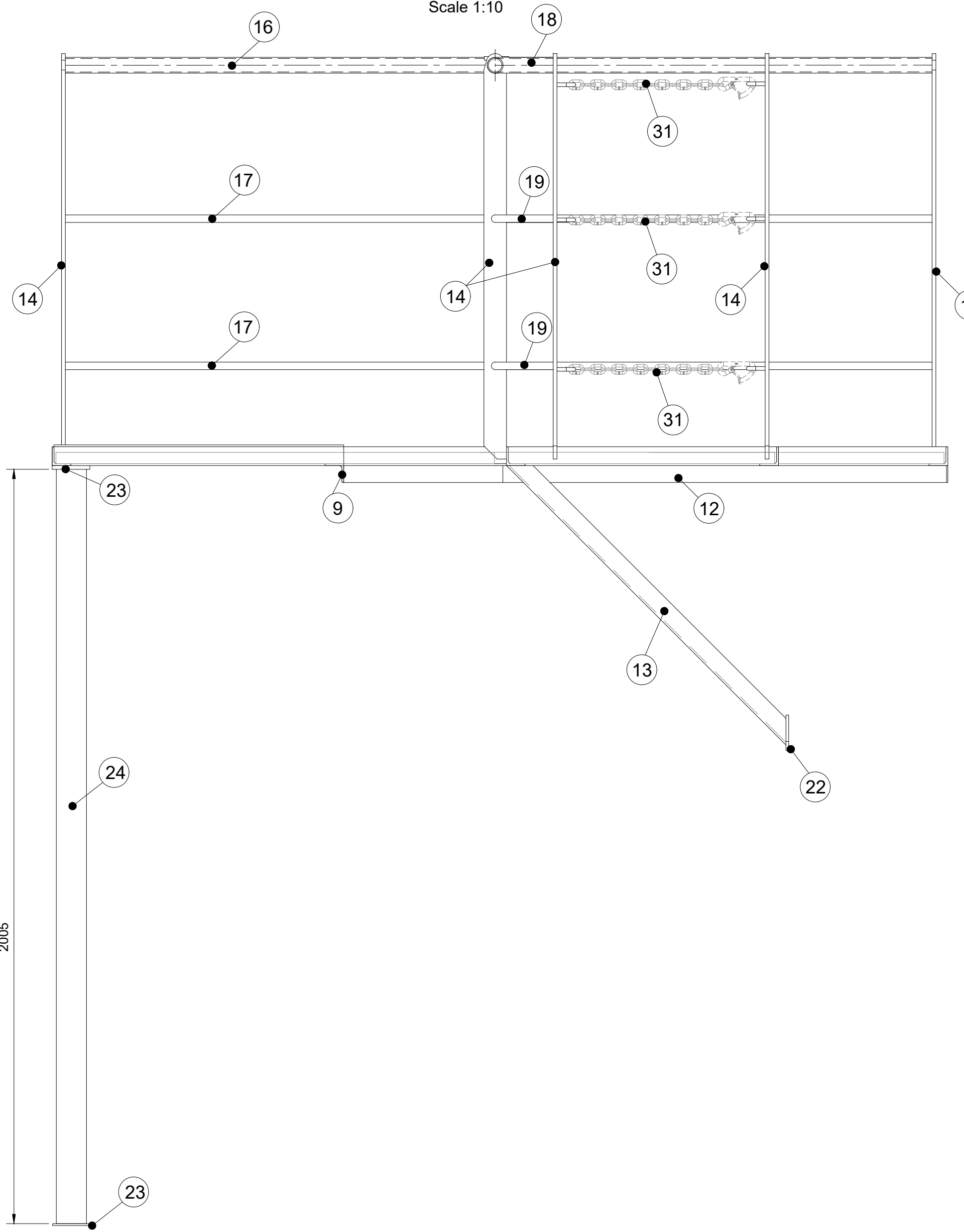
View B-B Scale 1:10
