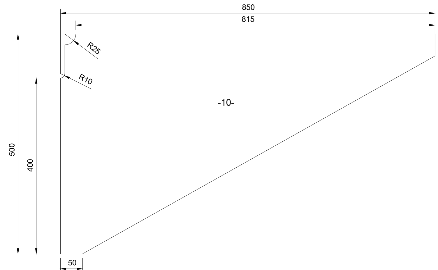
Scale 1:5
