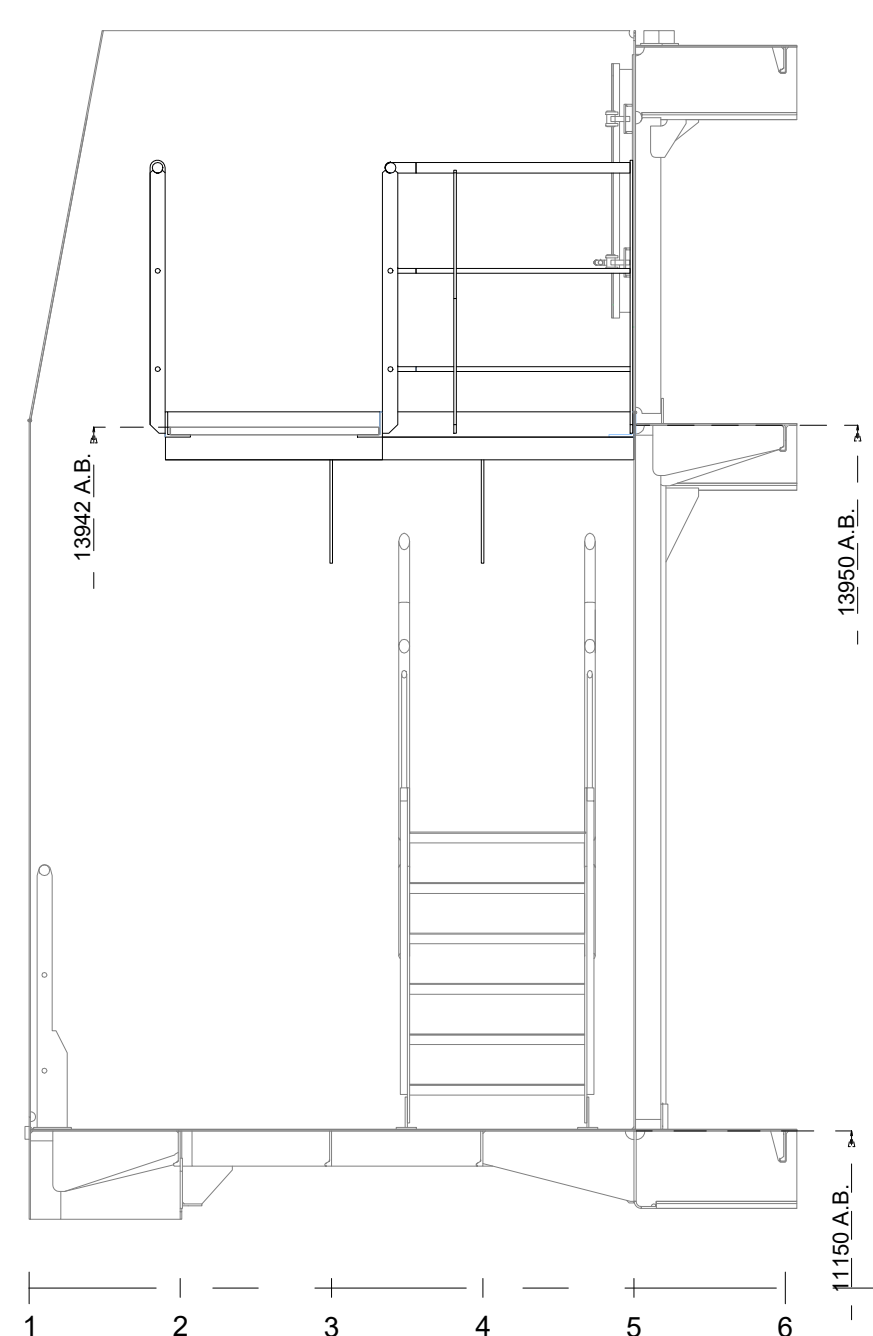
View section B-B
