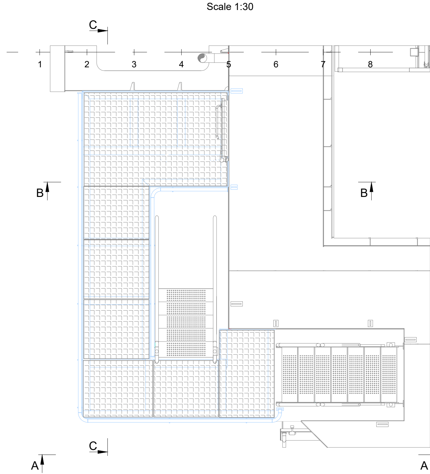
Top view platform and railing on Void deck
