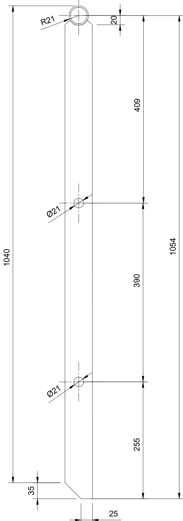
Detail Pos. 15 Scale 1:5
