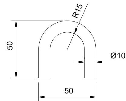
Detail Pos.28 Scale 1:2
