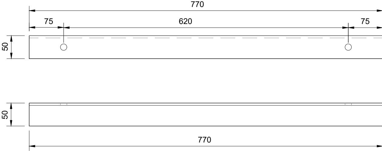
Detail Pos. 11 Scale 1:5
