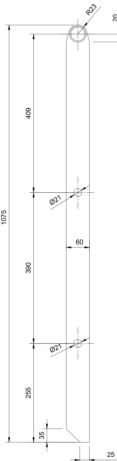
Detail Pos. 14 Scale 1:5
