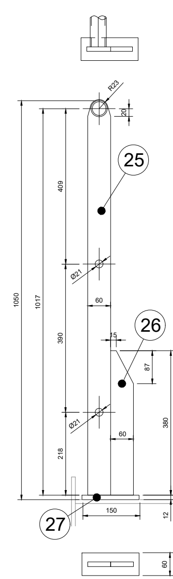
Detail Pos.25
