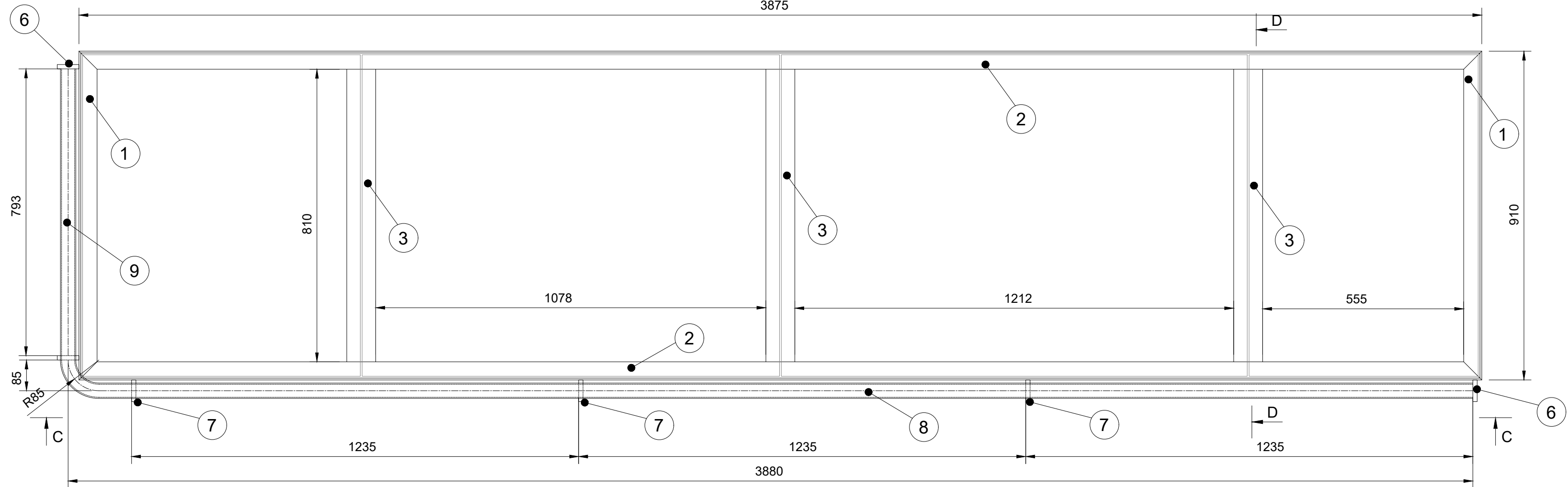
Top view platform and railing
