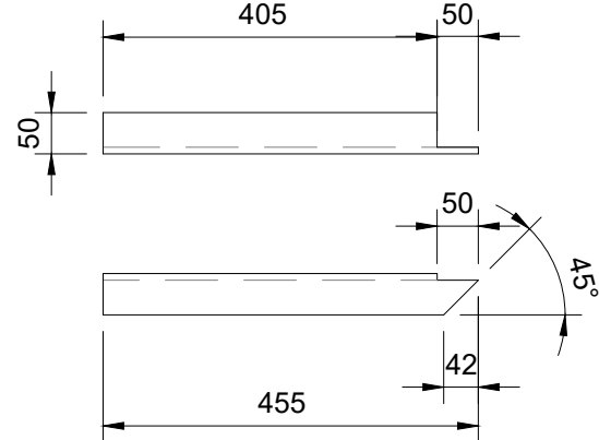
Detail Pos. 10 Scale 1:10
