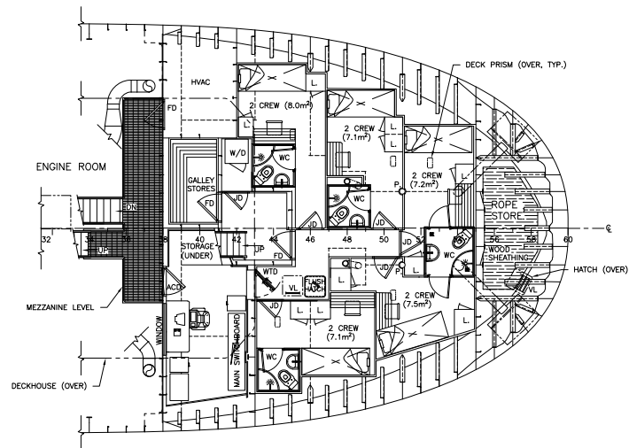
LOWER ACCOMMODATION PLAN
